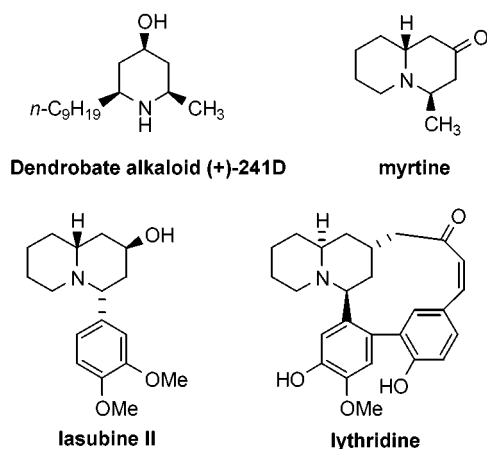
Figure 1. Structures of alkaloids possessing 2,4,6-trisubstituted piperidine moiety.
